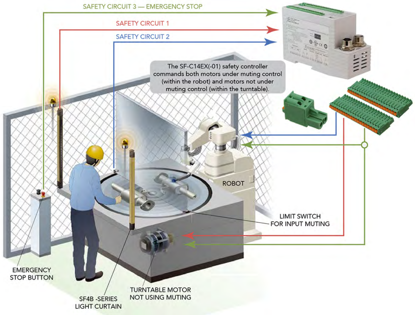
Figure 5: Safety controllers can unify multiple safety functions for flexible and reconfigurable safety installations. In the workcell illustrated here, the first safety circuit includes a light curtain that (upon reporting an interrupted status) opens a circuit switch to stop the turntable. The second safety circuit integrates muting controls that let the robot operate normally if a workpiece enters the workcell when the turntable is stopped. Otherwise, this circuit opens a switch to disable the robot. The third safety circuit includes an emergency stop that opens all switches and stops both turntable and robot. (Image source: Panasonic Industrial Automation Sales )
