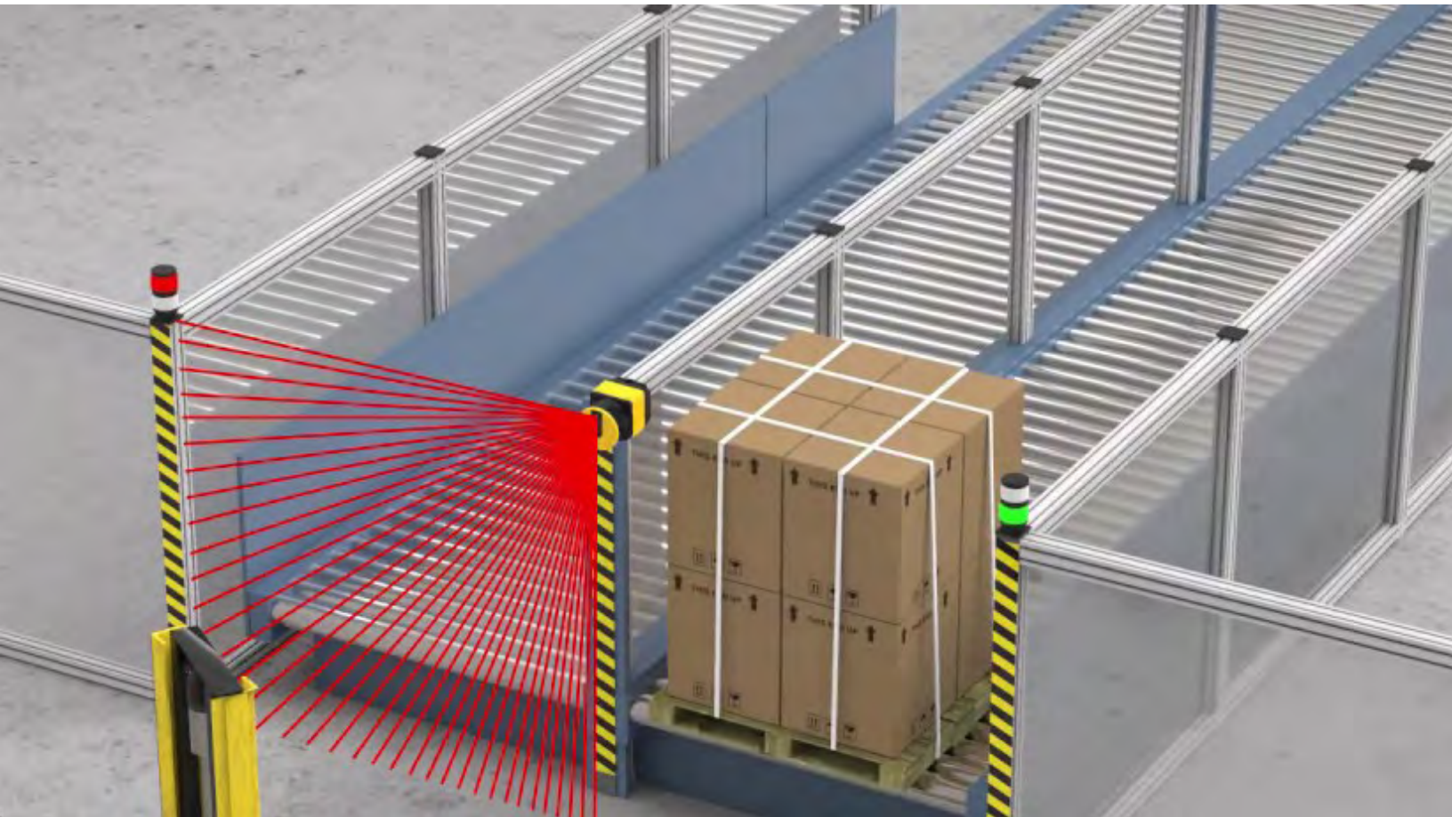
Figure 3: SX Series safety laser scanners from Banner Engineering can safeguard access points and areas in industrial applications. The device continuously scans 275° to protect personnel and machinery with warnings and safety zones customizable with free configuration software. Muting functions are also configurable in this software that, along with muting sensors networked to the SX Series scanner, eliminate the need for an additional module or controller. (Image source: Banner Engineering)
