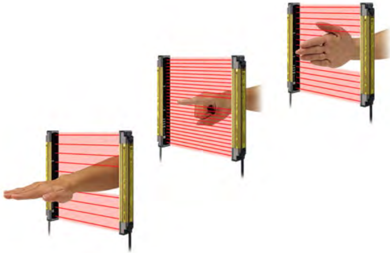
Figure 1: Safety light curtains control access to potentially hazardous areas in an industrial environment. The highest resolution (center) will detect the presence of a finger. Medium resolution (right) will sense a hand, while still lower resolution can be set to sense an arm or a whole person. (Photo credit: Omron STI)
