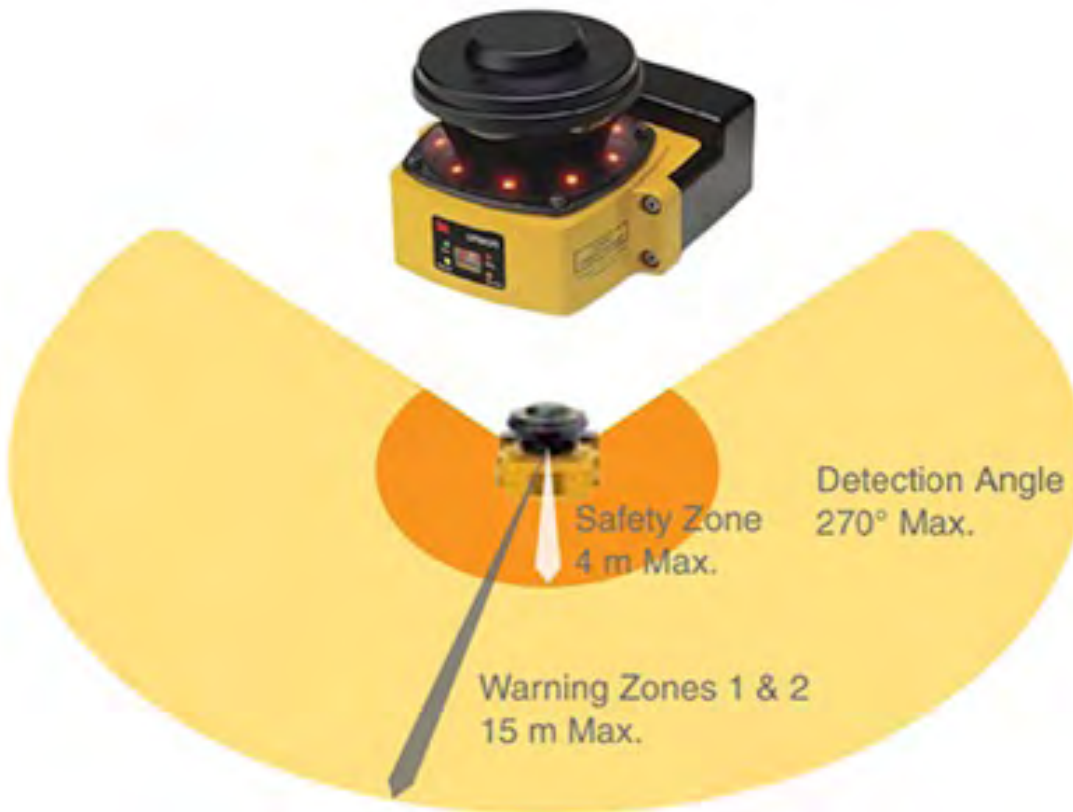
Figure 6: Omron's OS32C family of area scanners features multiple programmable zones (Image source: Omron Automation and Safety)
