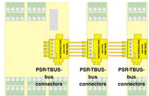
Figure 3: Adding safe I/O modules to extend the safety-monitoring system.
