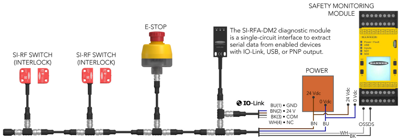
Figure 5: Innovative connectivity options have only increased the reliability of multi-guard installations in recent years. Here, an interface module is connected via T-adaptor networks to other safety components. (Image source: Banner Engineering )
