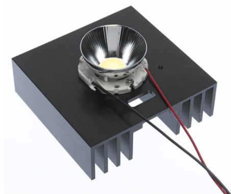
Molex LED Array Holder with Optic (optic sold separately from LEDIL)
