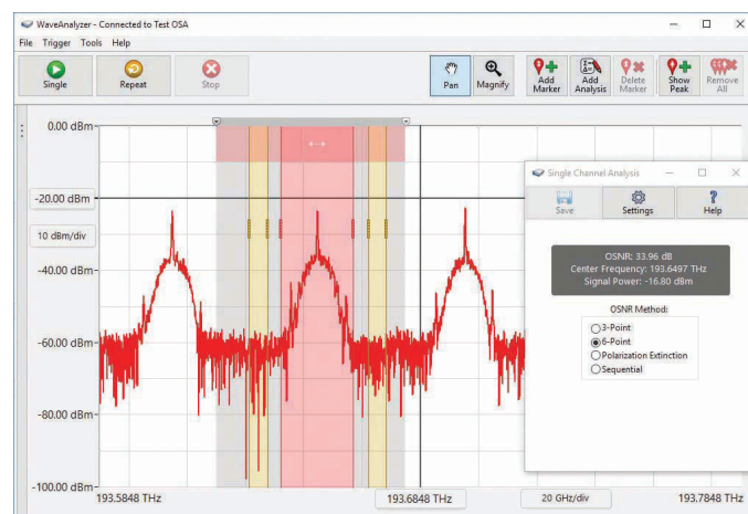
6-point OSNR measurement
