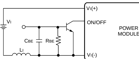
Figure 9. Properly Placing the Input Inductor.
