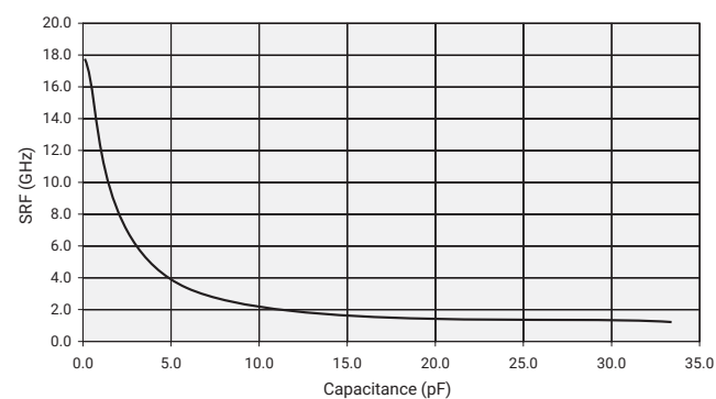
KAVX Accu-P® 0603 Capacitors SRF vs. Capacitance
