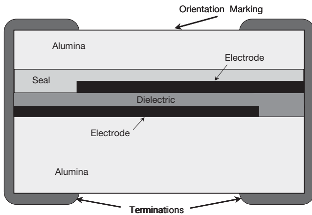
Figure 3. Accu-P® Capacitor Structure
