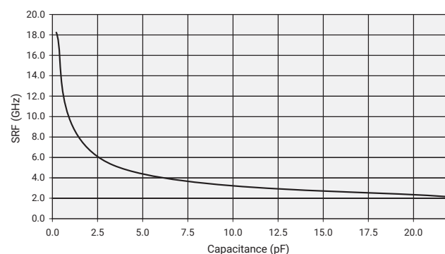
KAVX Accu-P® 0603 Capacitors SRF vs. Capacitance
