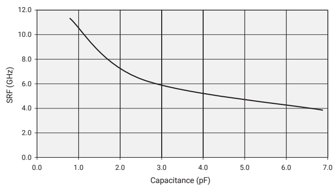
KAVX Accu-P® 0402 Capacitors SRF vs. Capacitance
