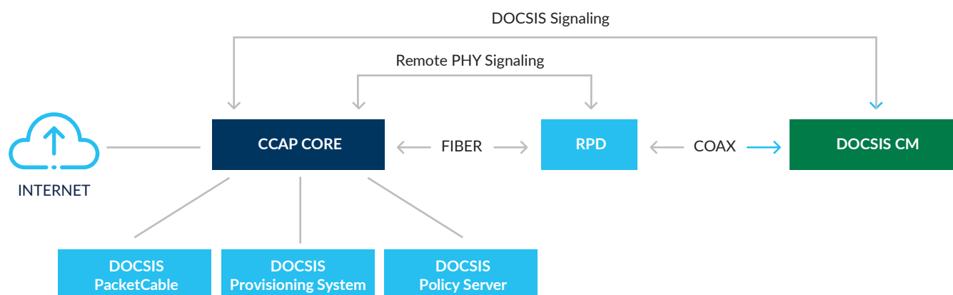
Figure 1 Remote PHY architecture (CableLabs)
