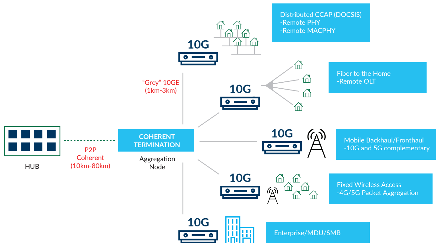
Figure 3 10G CableLabs architecture (from CableLabs website)
