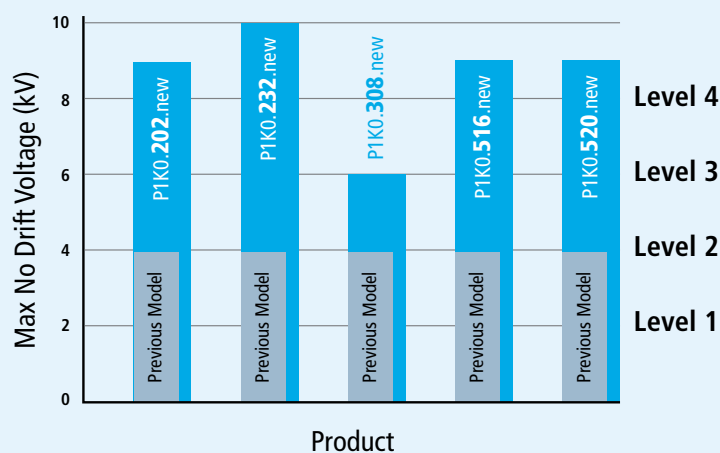
ESD Test Levels (IEC/EN 61000-4-2)
