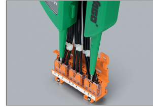
Testing connectors via their front test slots, which remain accessible when mounted
