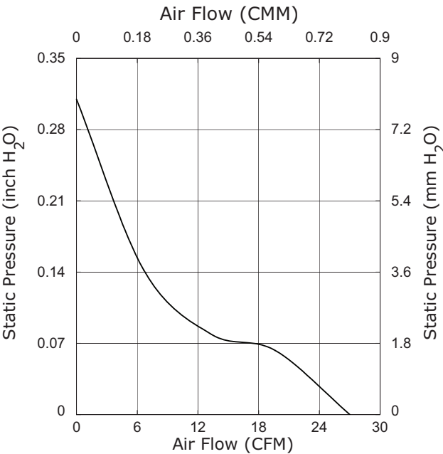
CFM-6025V-252-312
