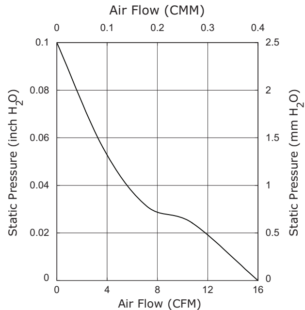
CFM-6025V-231-167
