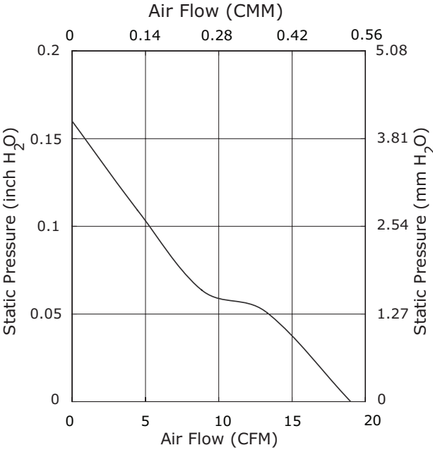
CFM-6025V-125-107
