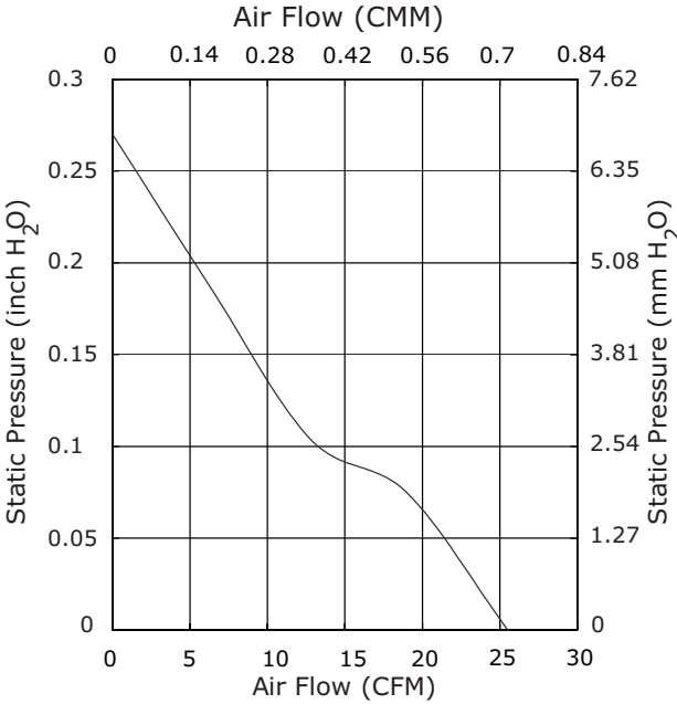
CFM-6025V-131-167
