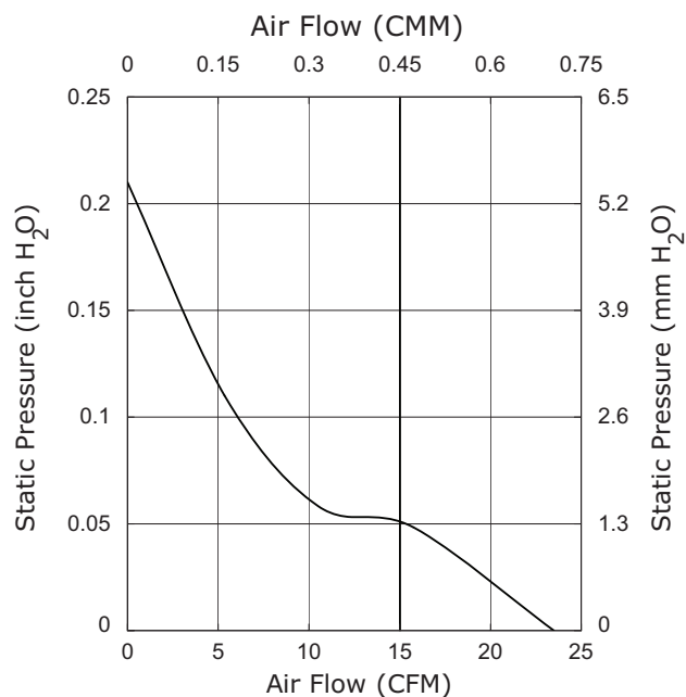
CFM-6025V-145-270
