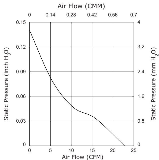
CFM-6015V-139-292
