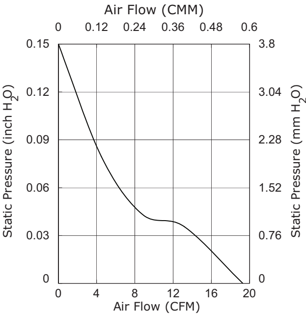
CFM-6025V-238-220
