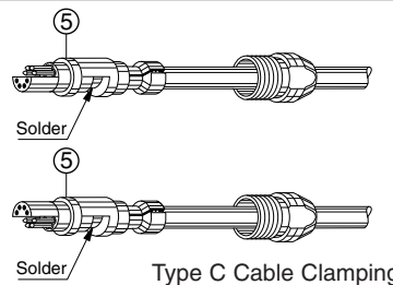
Type C Cable Clamping
