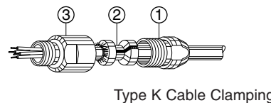
Type K Cable Clamping
