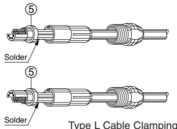
Type L Cable Clamping
