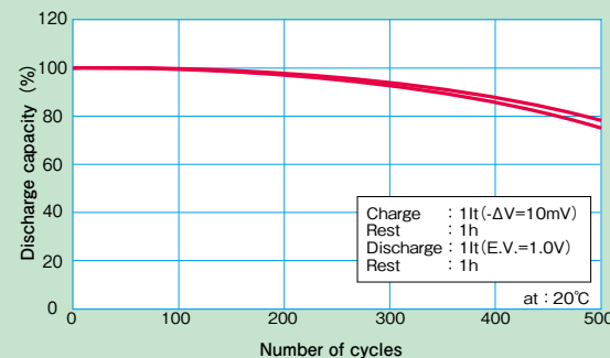
● Charge/Discharge Cycle Characteristics
