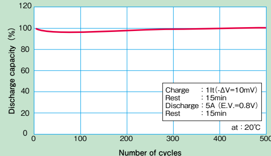
● Charge/Discharge Cycle Characteristics ● 充放電サイクル特性
