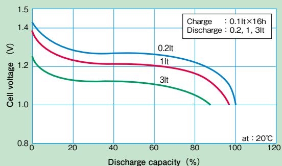
● Discharge Characteristics
