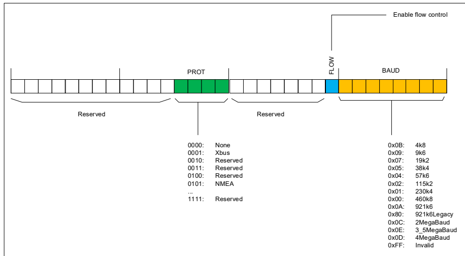
Figure 2 Port Configuration
