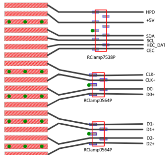
HDMI Type A Connector
