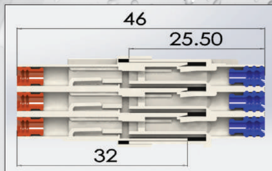
Assembly Layout
