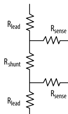
Figure 7: Kelvin principle measurement
