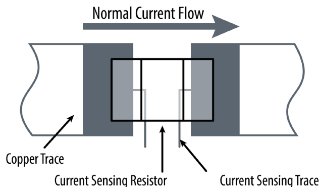
Figure 8: 2-Terminal CSR with the 4-wire Kelvin principle
