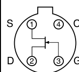
TO-72 TOP VIEW
