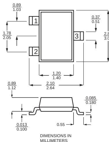
SOT-23 3 Lead
