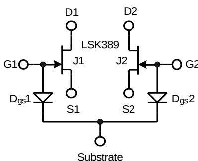
Figure 8: LSK389 including substrate diodes
