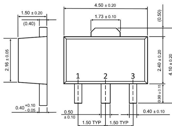
SOT-89 3 Lead
