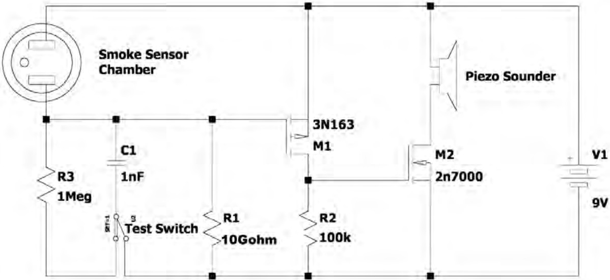
Simplest Possible Smoke Detector
