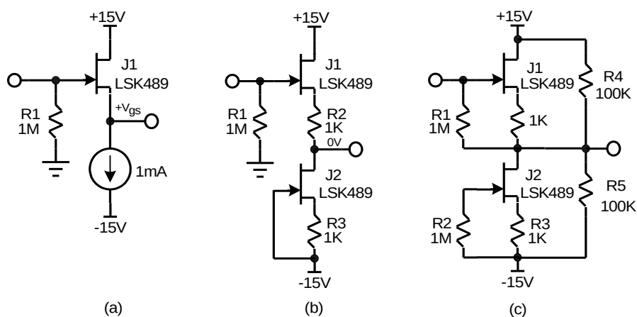
Figure 3: LSK489 Source Followers
