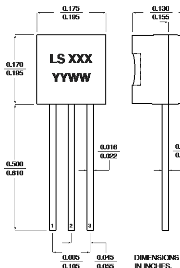
TO-92 3 Lead
