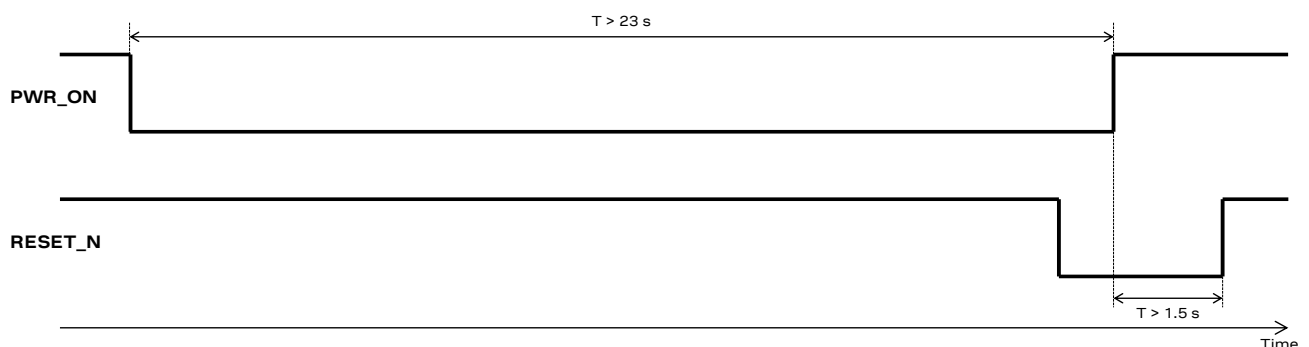
Figure 6: PWR_ON and RESET_N lines waveforms timings to perform an abrupt emergency hardware shutdown
