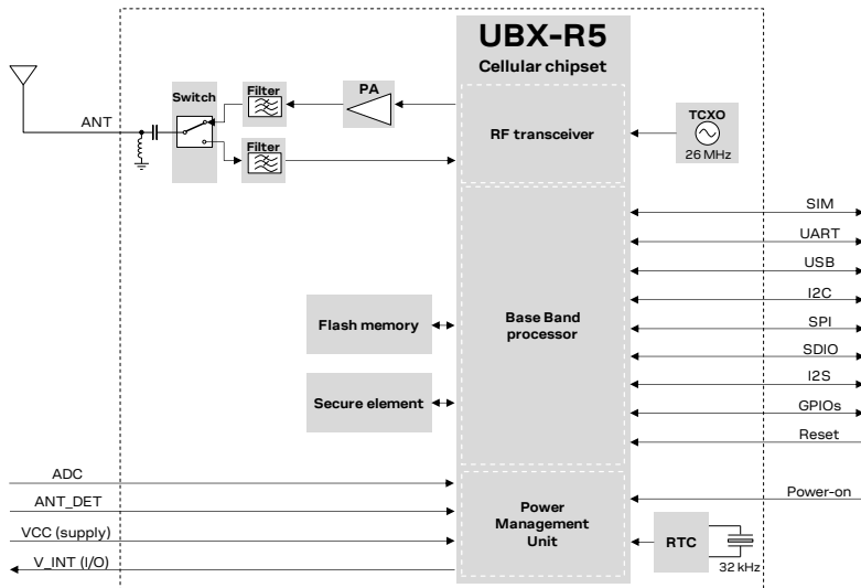
Figure 3: SARA-R510S block diagram 1
